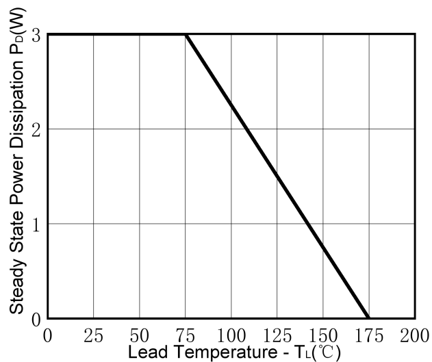
Steady State Power Dissipation Derating Curve
